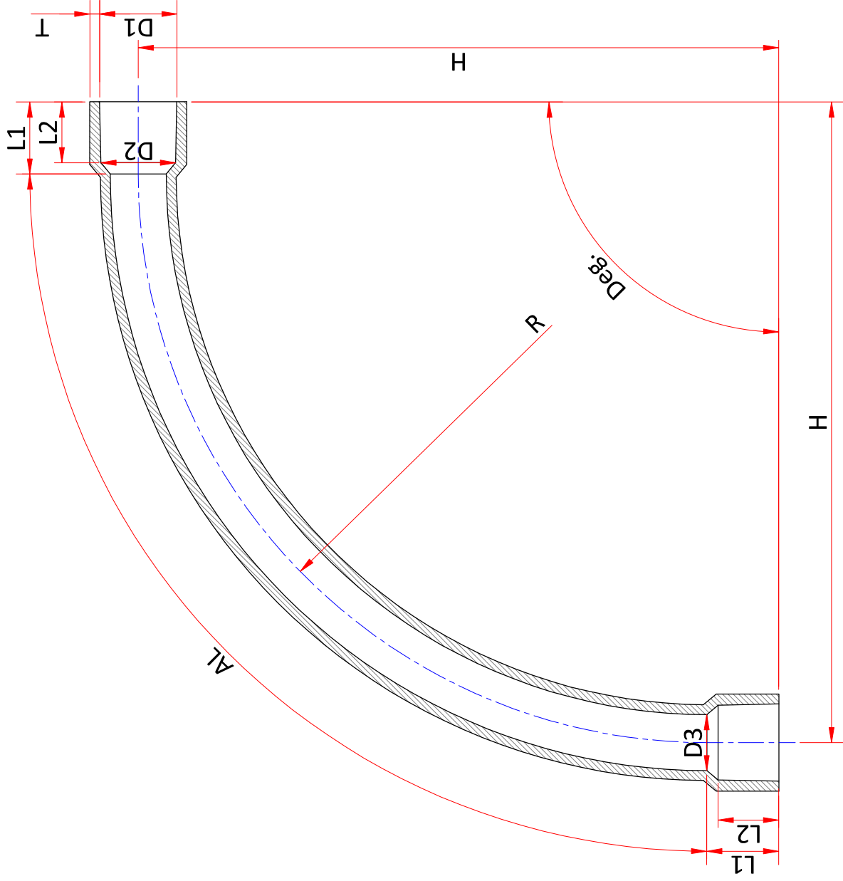
DIMENSION TABLE
