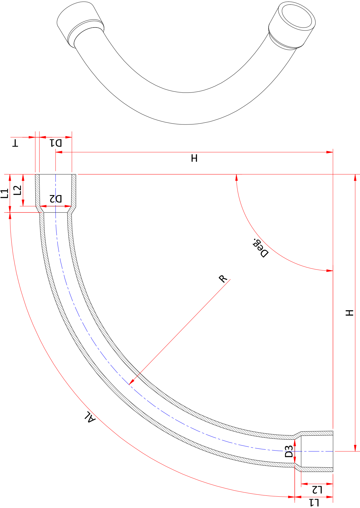
DIMENSION TABLE
