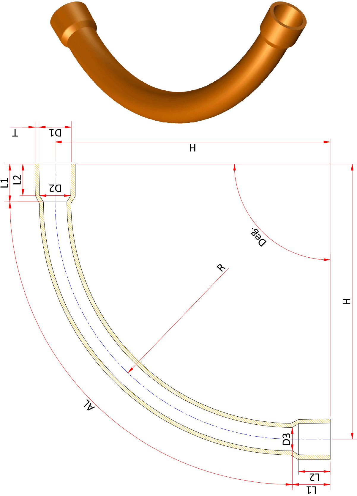
DIMENSION TABLE
